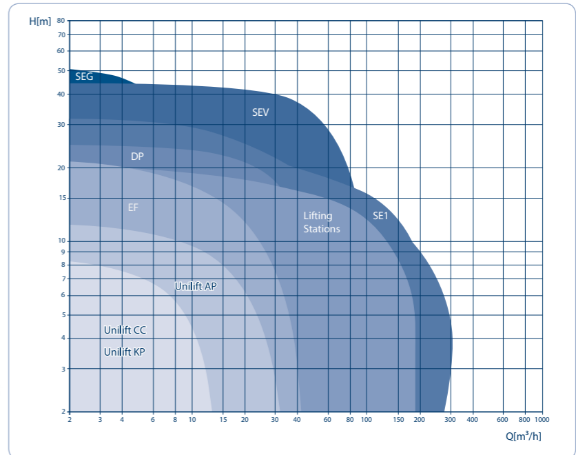
Pump performance
