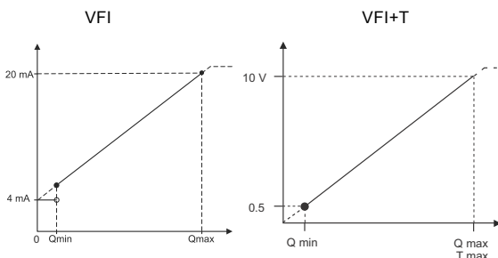
Fig. 16 Flow response
