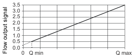
Fig. 68 Flow response in Analogue mode
