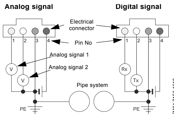
Fig. 33 Electrical connections
