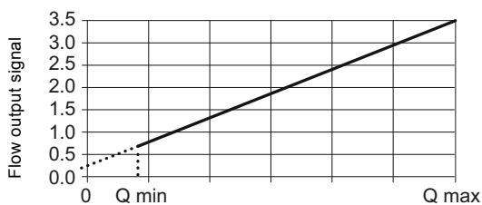
Fig. 96 Flow response in Analogue mode
