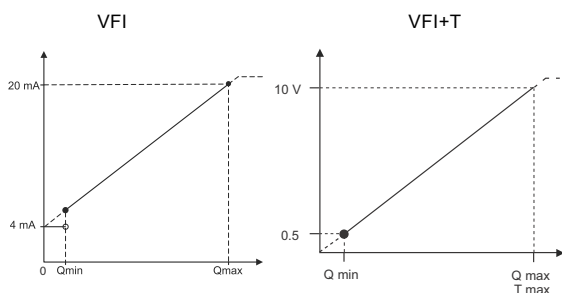
Fig. 13 Flow response
