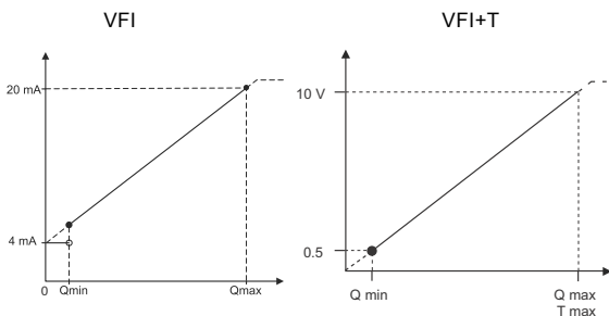
Fig. 28 Flow response
