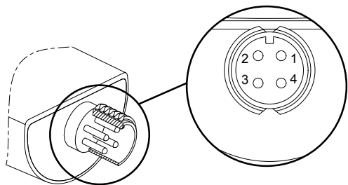
Fig. 6 Electrical connections
