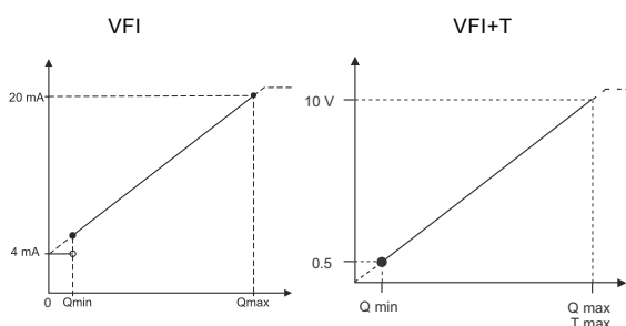
Fig. 19 Flow response
