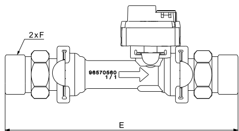
Fig. 90 Dimensions, MFS 4-40 l/min, with adapter
