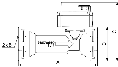
Fig. 43 Dimensions, VFS, 2-40 l/min, without adapter
