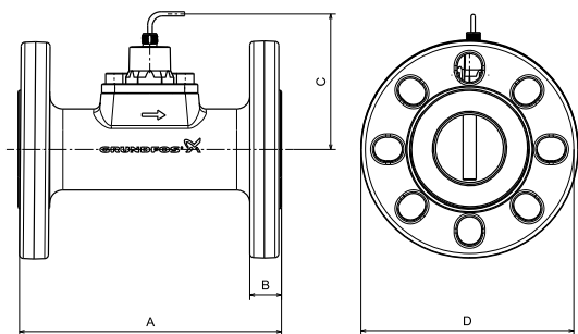
Fig. 30 Dimensions, VFI with flanges
