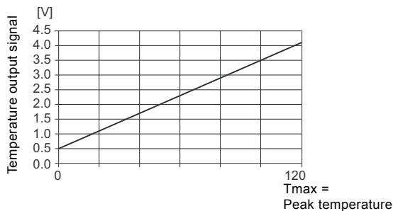
Fig. 41 Temperature response in Analogue mode
