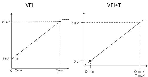
Fig. 31 Flow response
