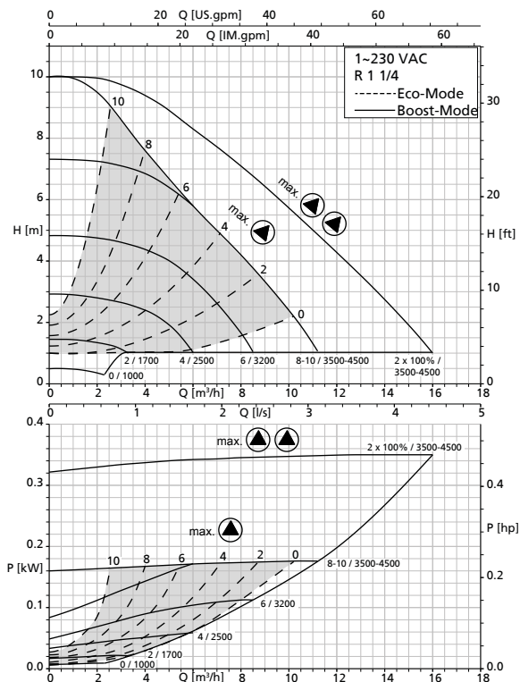
Calio Z 30-100 modes Boost + Eco
