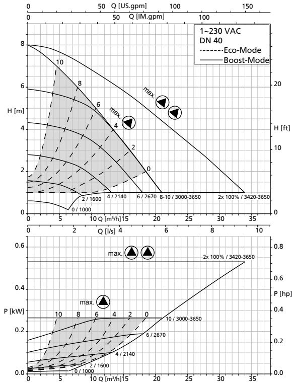
Calio Z 40-80 modes Boost + Eco
