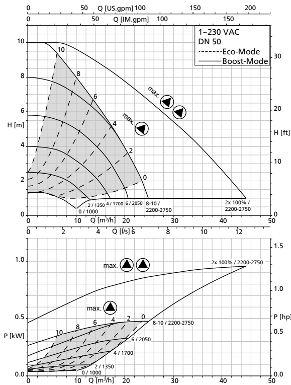
Calio Z 50-100 modes Boost + Eco
