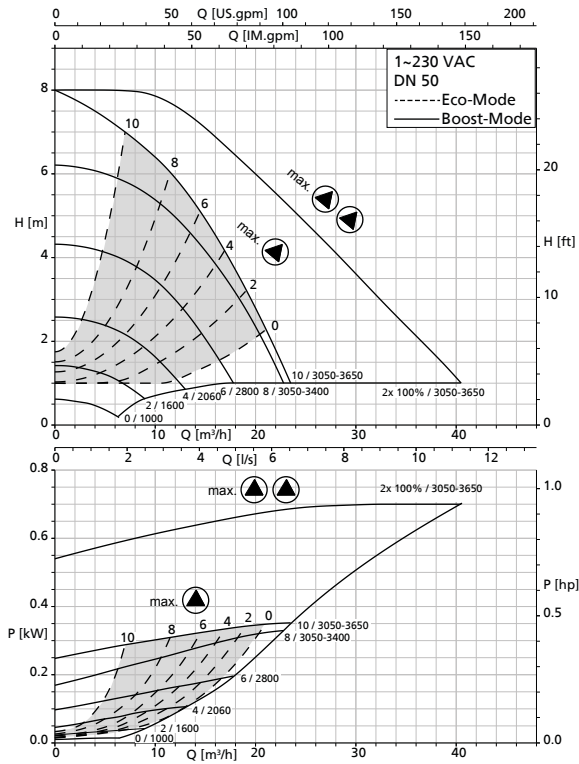
Calio Z 50-80 modes Boost + Eco
