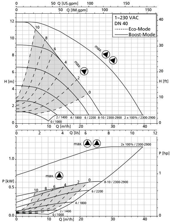
Calio Z 40-120 modes Boost + Eco
