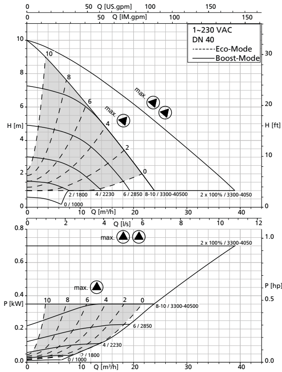
Calio Z 40-100 modes Boost + Eco
