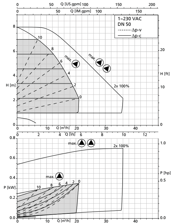
Calio Z 50-80 Δpv + Δpc
