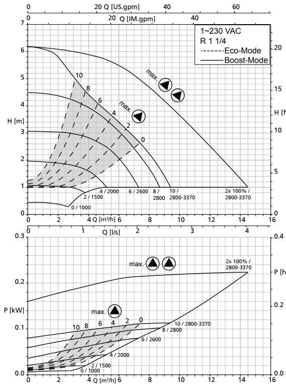
Calio Z 30-60 modes Boost + Eco
