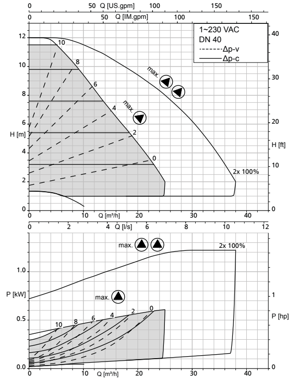
Calio Z 40-120 Δpv + Δpc
