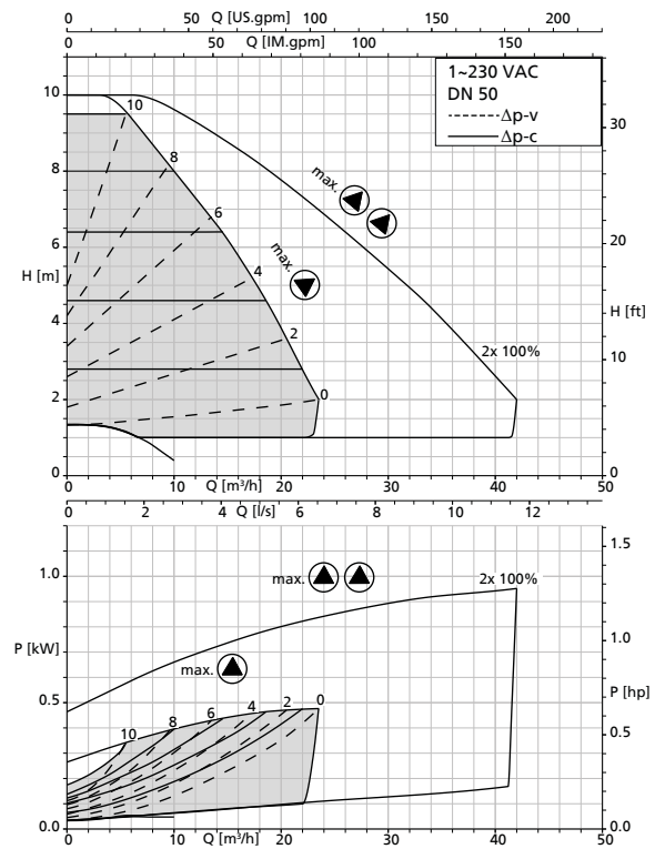
Calio Z 50-100 Δpv + Δpc
