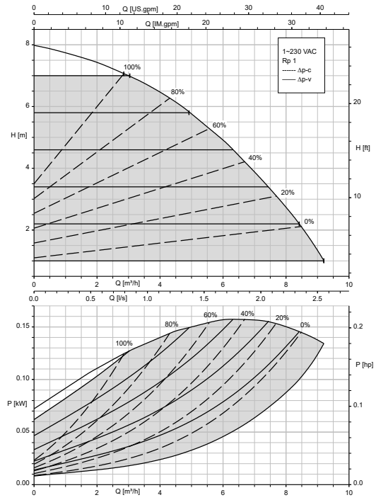
CalioTherm Pro 25-80 \Delta p_v , \Delta p_c
