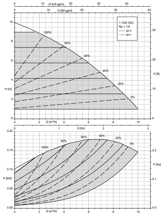
CalioTherm Pro 30-100 \Delta p_v , \Delta p_c
