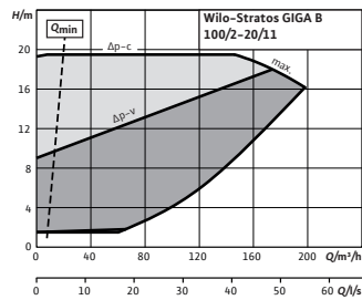
Wilo-Stratos GIGA B 100/2-20/11
