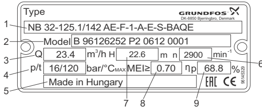
Fig. 5 Example of nameplate
