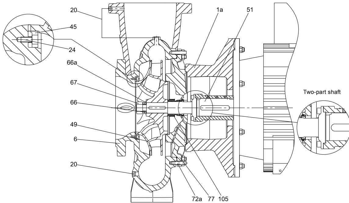
Fig. 7 Sectional drawing, tangential outlet, DN 200 and DN 250
