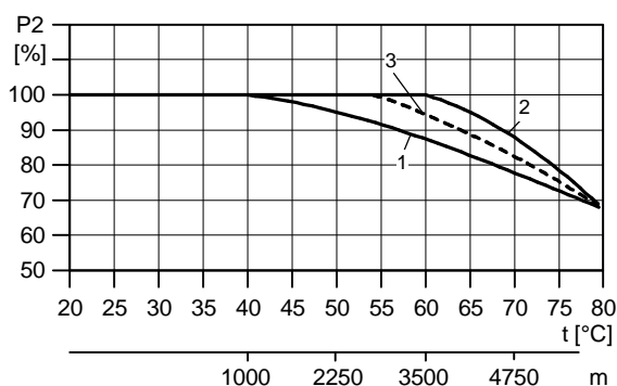
Fig. 32 Maximum motor output in relation to ambient temperature and altitude
