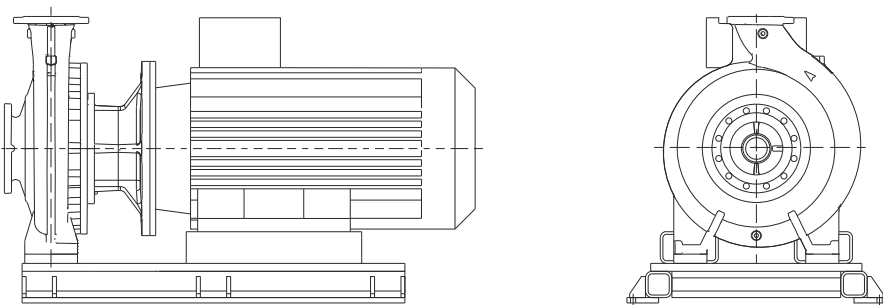
Fig. 69 NB pump with base frame
