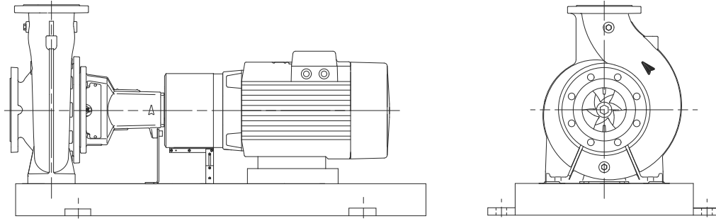
Fig. 63 NK pump with EN/ISO base frame
